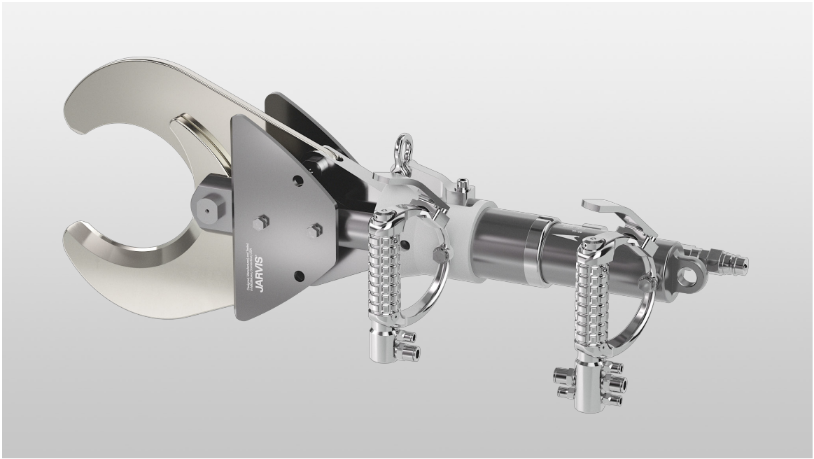
30CL 30CL-1: fore and hind beef hock and horn cutters 30CL-3: horn cutter for sheep, goats and beef nubs
