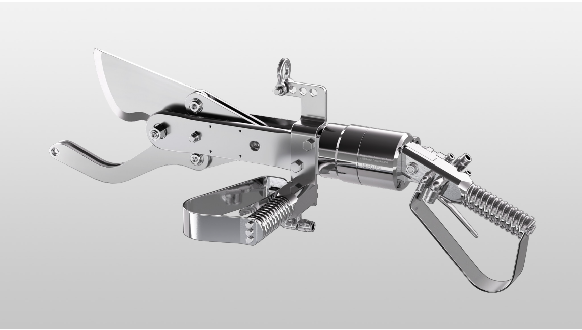
ABC-1 Hydraulic powered aitch bone cutter for hogs
